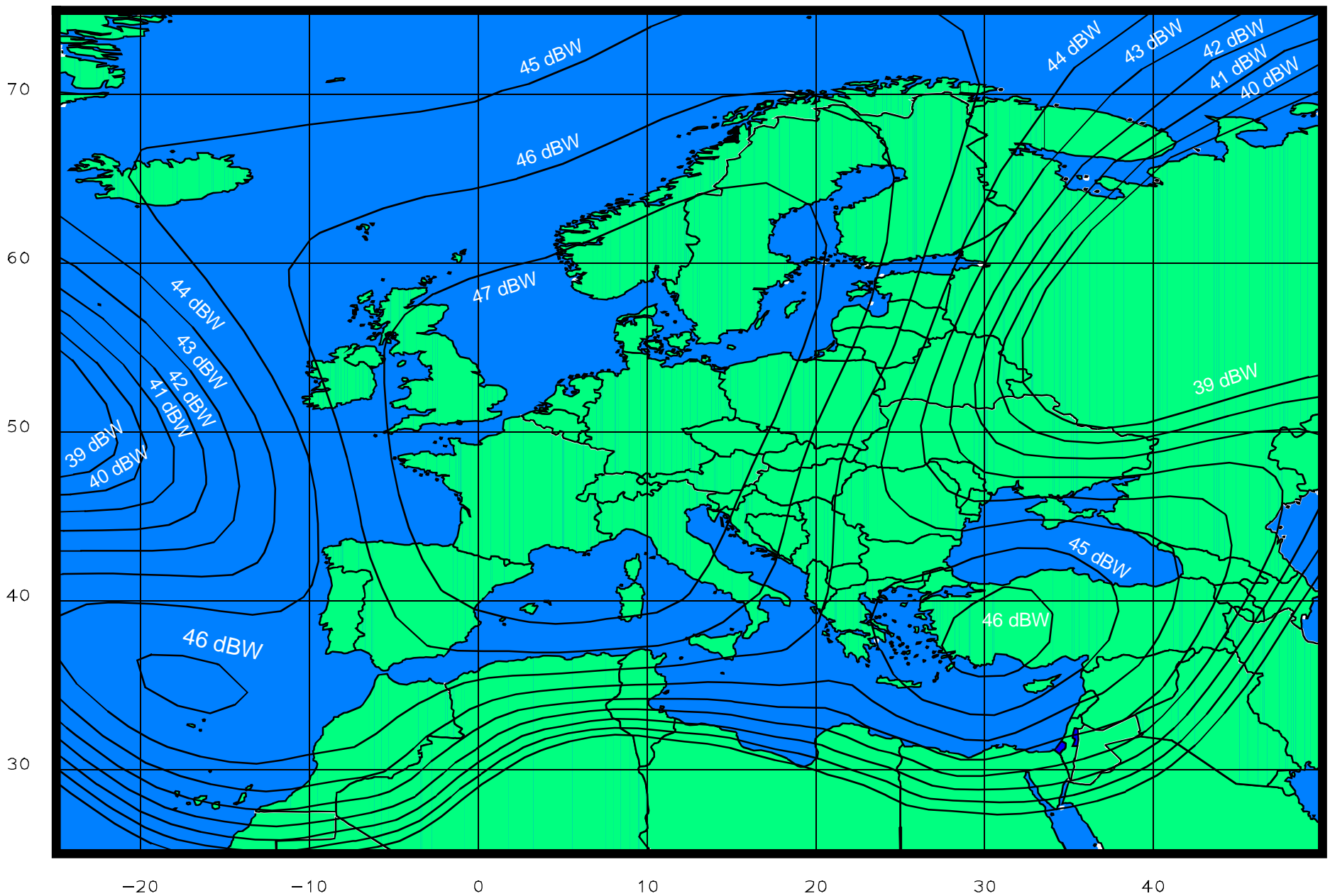
Figure 3: Transponders 20, 21 and 22, Widebeam coverage (EUTELSAT II-F1)
